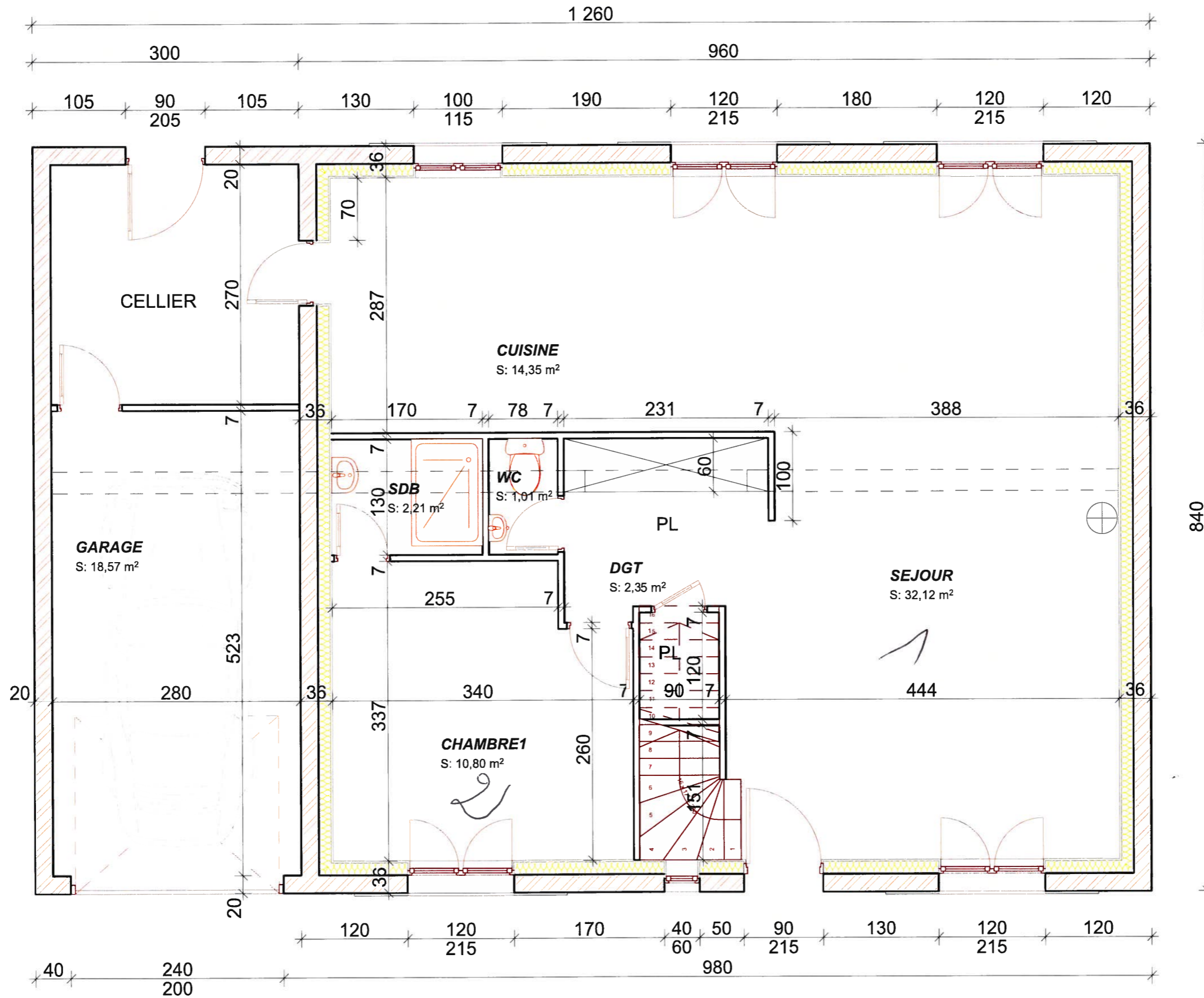
REZ DE CHAUSSEE SURFACE HABITABLE: 62.82 m 2 SURFACE GARAGE: 18.57
